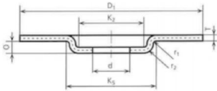
Grinding wheel with depressed center
