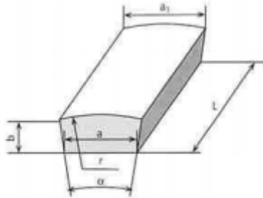
Grinding segment without thread
