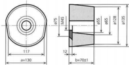
Grinding segment with thread
